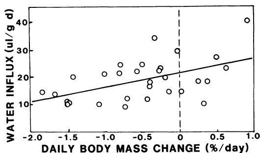
Fig. 2. Least squares linear regression relation between water influx rate ( \mu\text{L H}_2\text{O/g.d.} ) and daily body mass change (% body mass change per day). Water influx = 5.341 [\% \text{ body mass change per day}] + 21.78 ( r^2 = 0.261 , F_{(1,28)} = 9.87 , P < .005 ).
