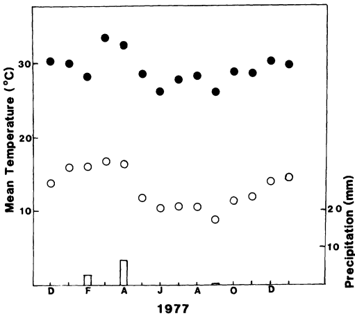
Fig. 1. Daily mean maximum (closed circles) and minimum (open circles) temperature and monthly precipitation (fog and rain) of Gobabeb between Dec. 1976 and Jan. 1978.
